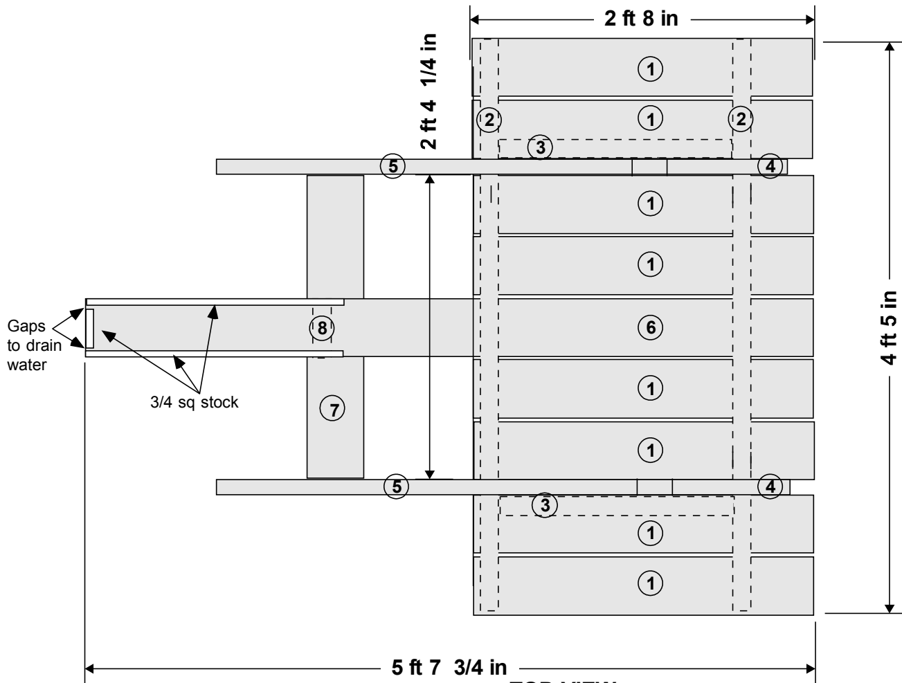
TOP VIEW
